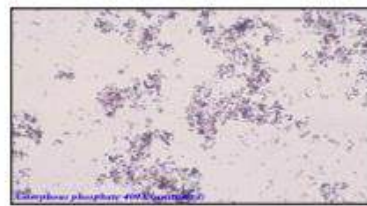
Amorphous Phosphates
